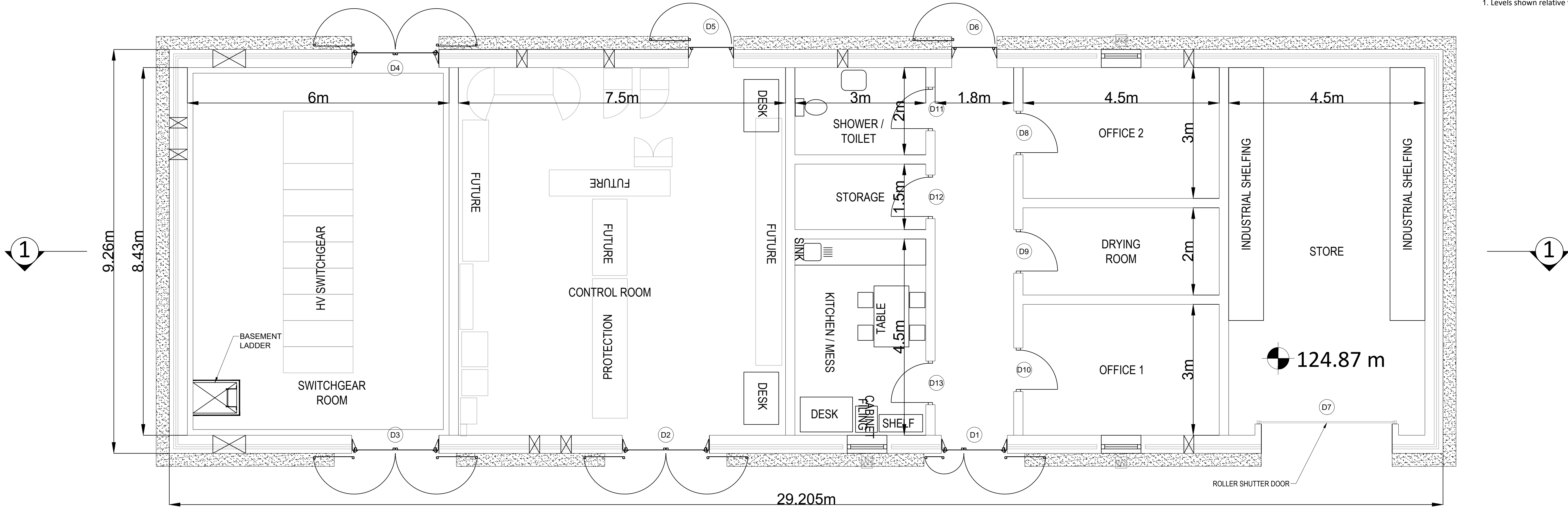
BUILDING PLAN Scale: 1:50
