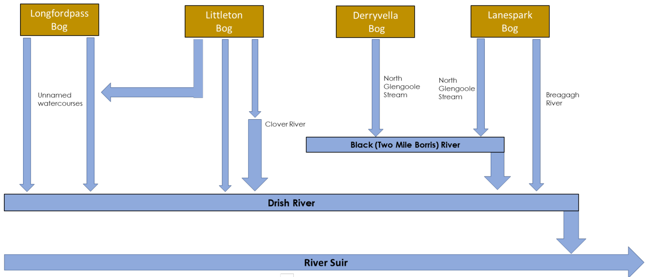
Figure 2-2: Hydrological Flowpaths for the Site
